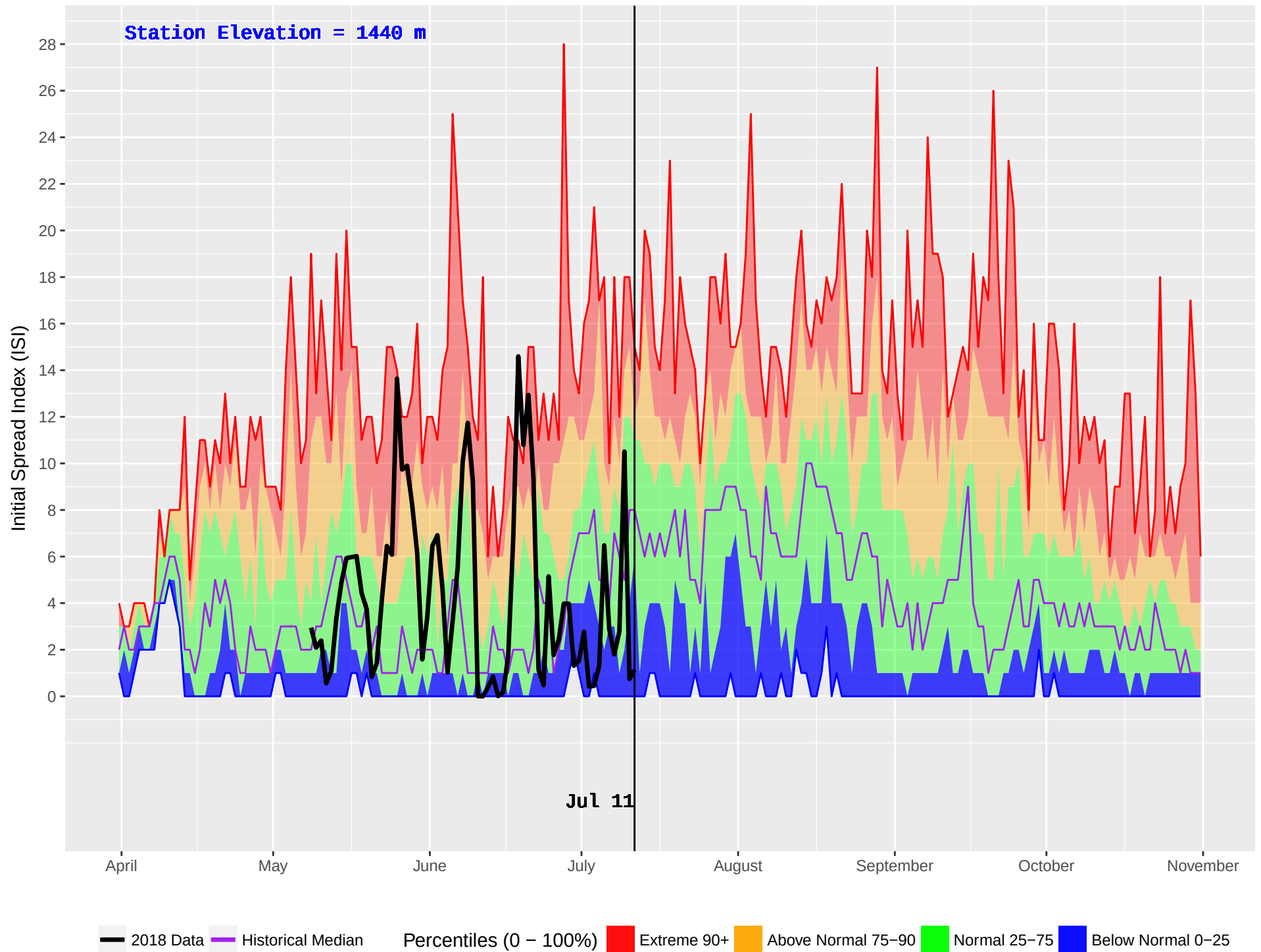
PASKA LAKE (326) : Historical (1999–2016) and Current (2018) Noon Initial Spread Index (ISI)
