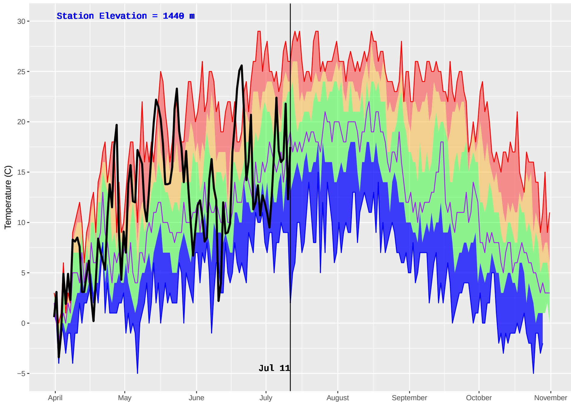
PASKA LAKE (326) : Historical (1999–2016) and Current (2018) Noon Temperature
