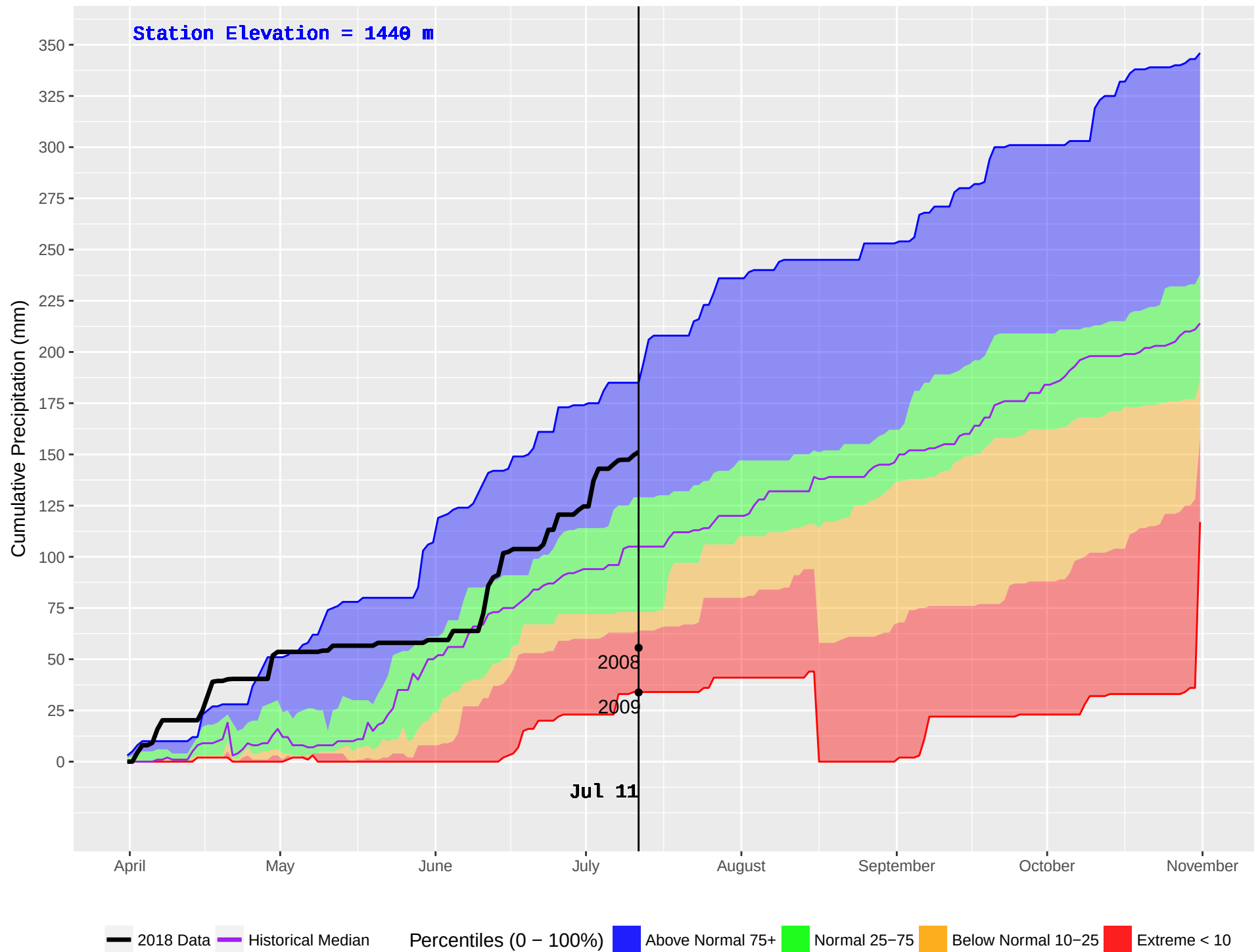
PASKA LAKE (326) : Historical (1999–2016) and Current (2018) Noon Cumulative Precipitation
